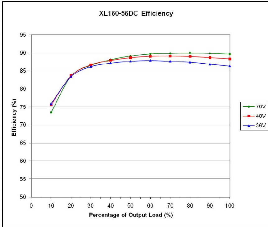
Figure 5-28 Efficiency of XL160-56DC (Non Current Sharing)
