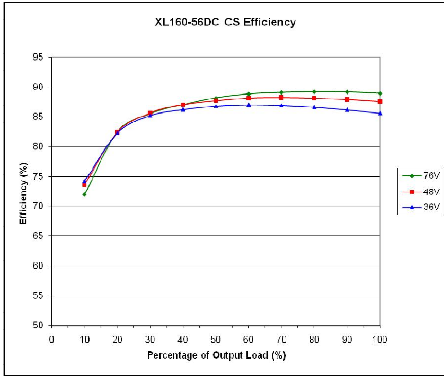
Figure 5-27 Efficiency of XL160-56DC CS (Current Sharing)
