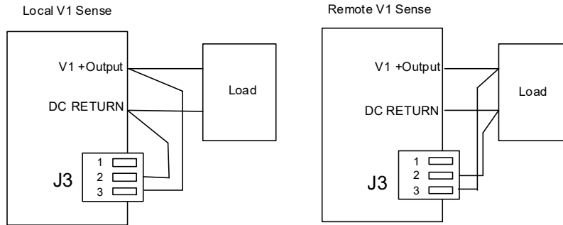
Figure 3-4 Remote Sensing Wiring: XL125/XL160-05DC [CS]
