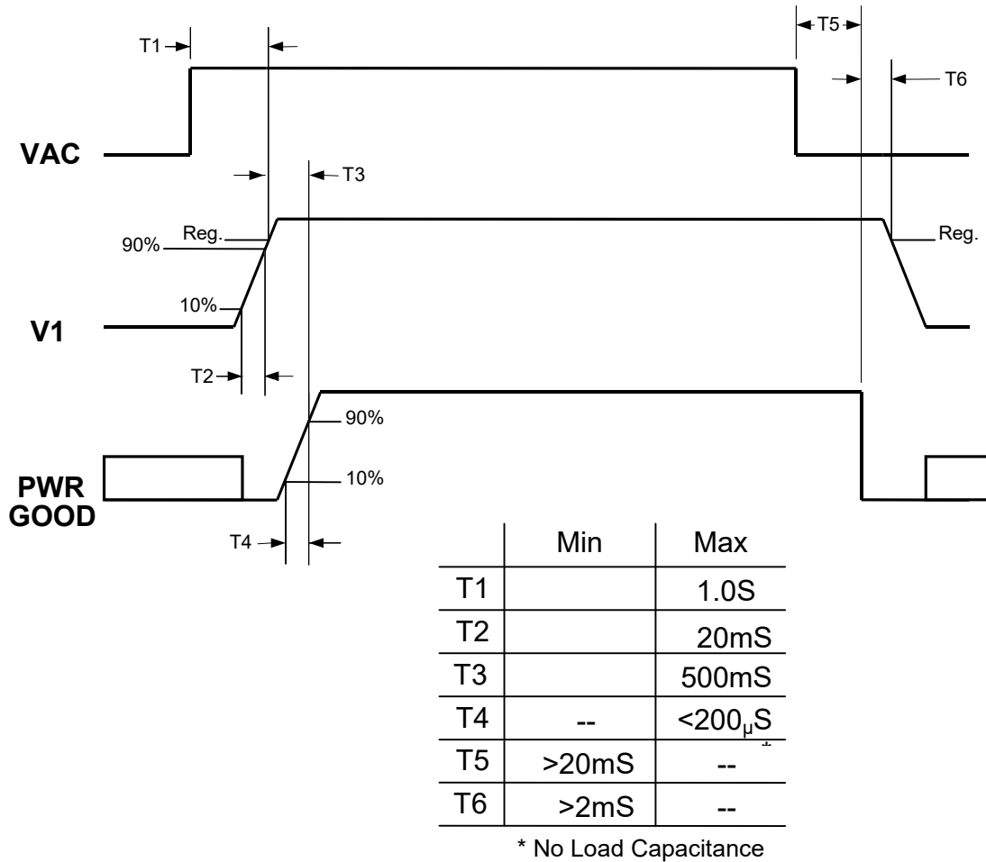
Figure 6-1 Timing Diagram
