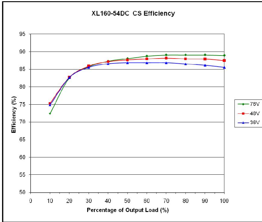
Figure 5-25 Efficiency of XL160-54DC CS (Current Sharing)
