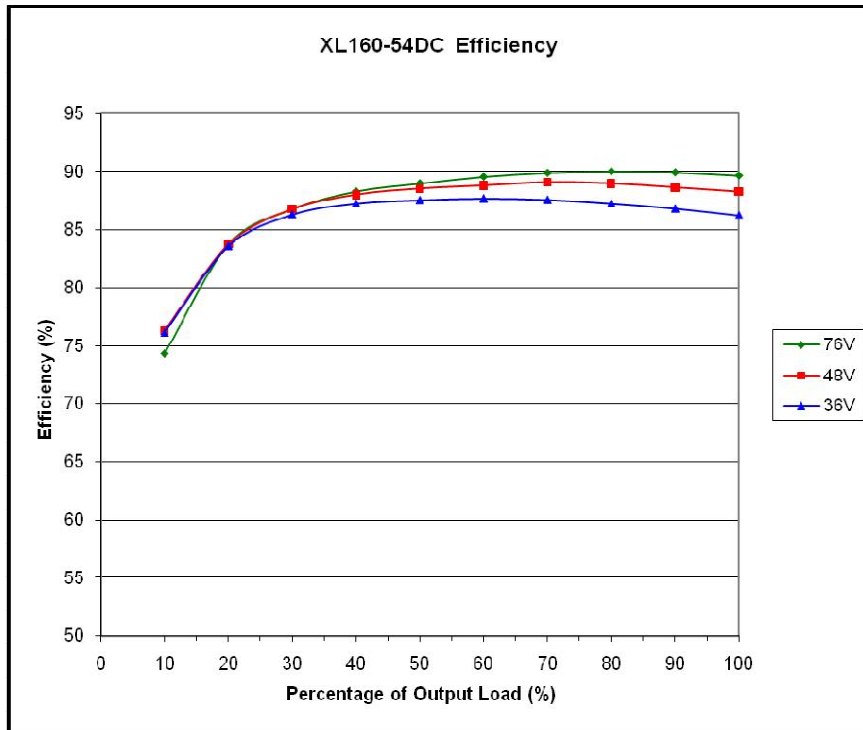
Figure 5-26 Efficiency of XL160-54DC (Non Current Sharing)
