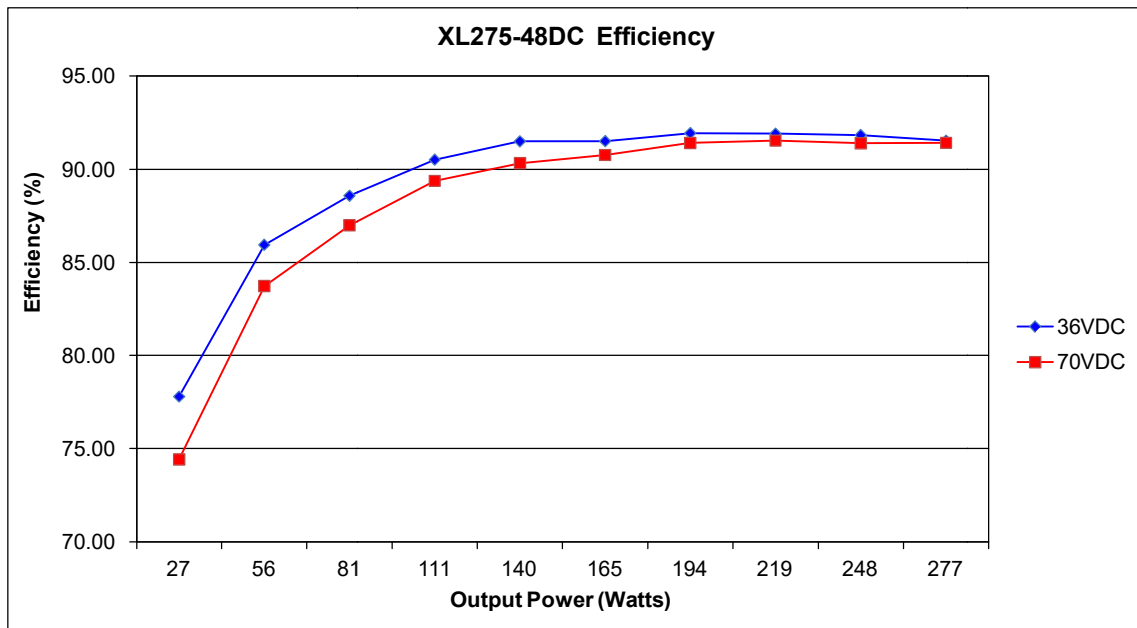
Figure 3-3 XL275-48DC Efficiency
